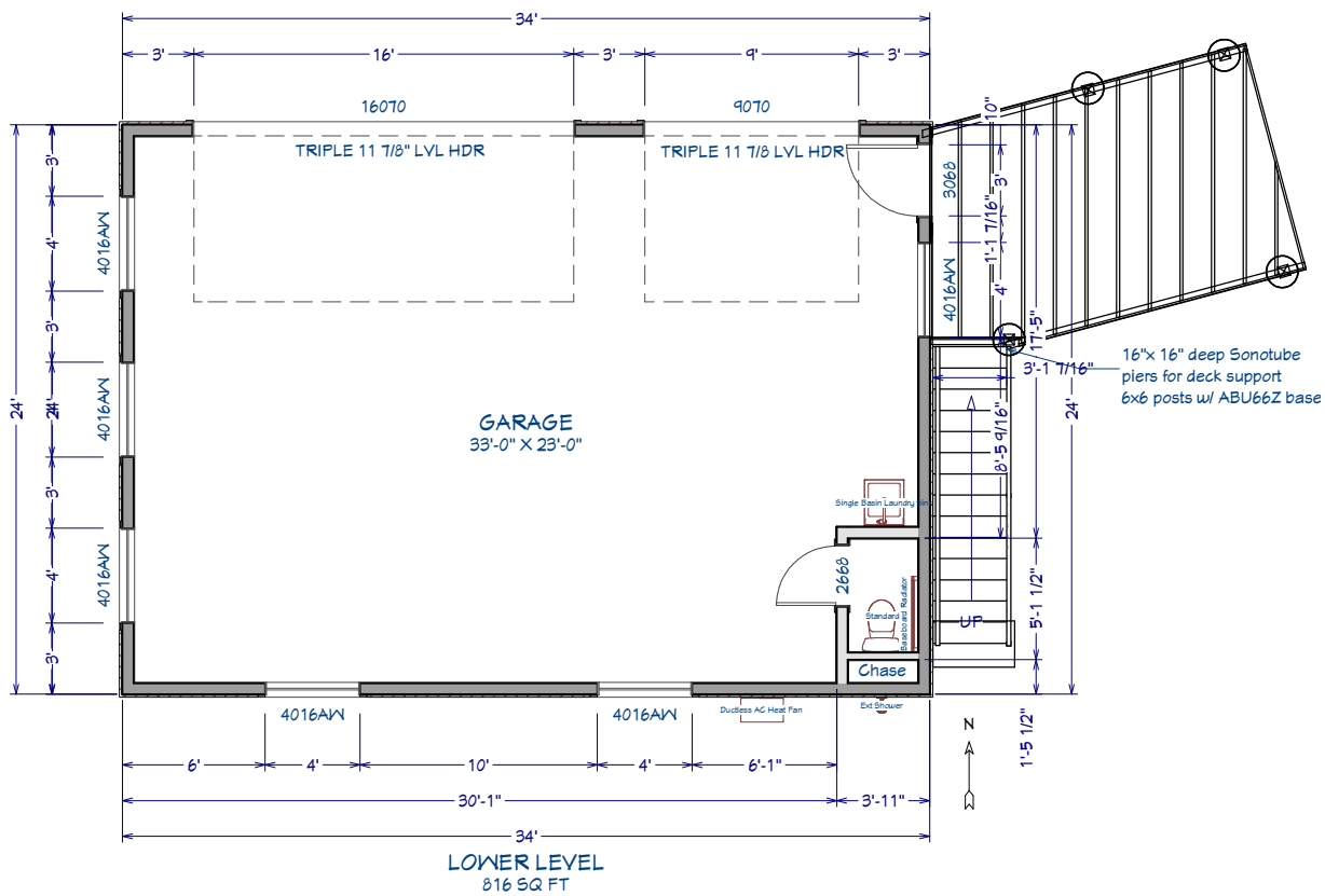
1st Floor
